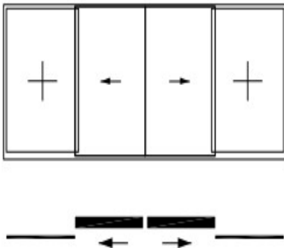
Picture: 7 Flying telescopic system
