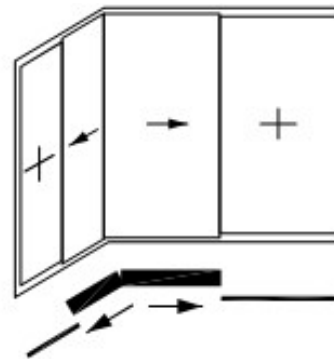
Picture: 12 Open Corner with external sashes
