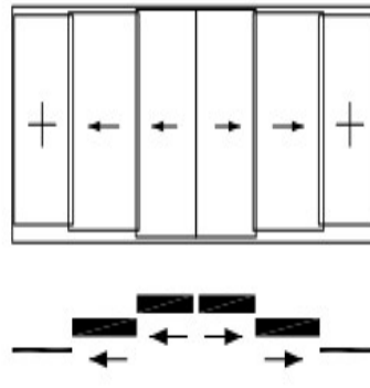
Picture: 12 Open Corner with external sashes
