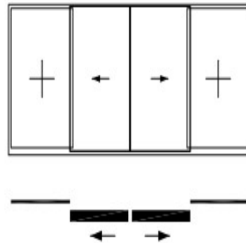
Picture: 6 Telescopic system with 2 internal sashes
