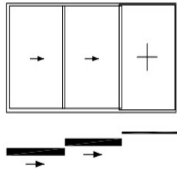
Picture: 6 Telescopic system with 2 internal sashes
